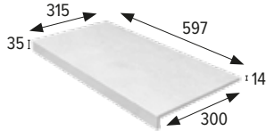
Straight stair-tread 60
